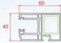
Yan Ray Profili
